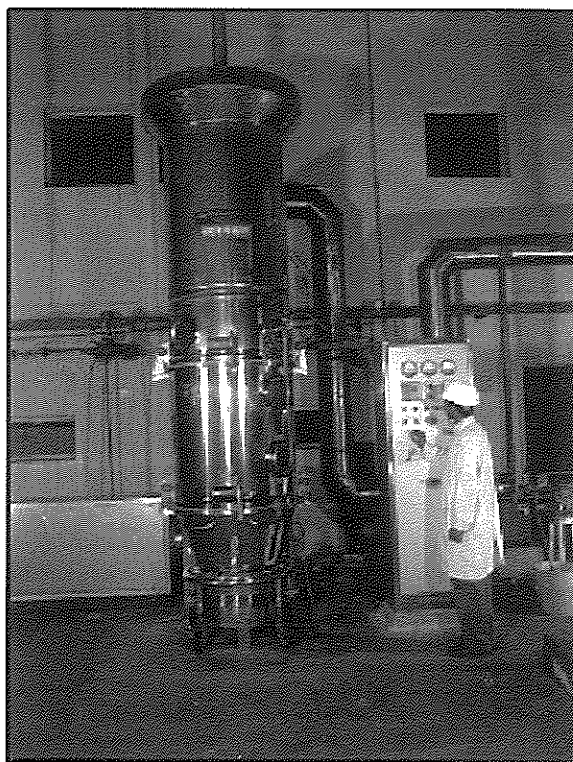
Spray Granulator
